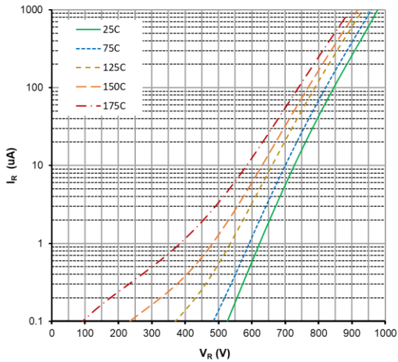
Figure 3. Reverse Characteristics
