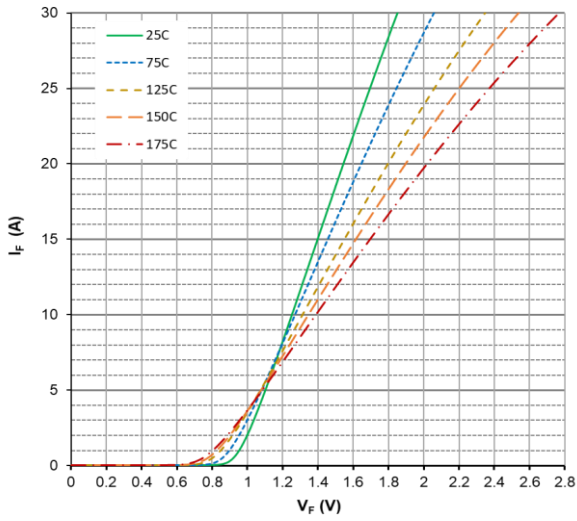
Figure 1. Forward Characteristics
